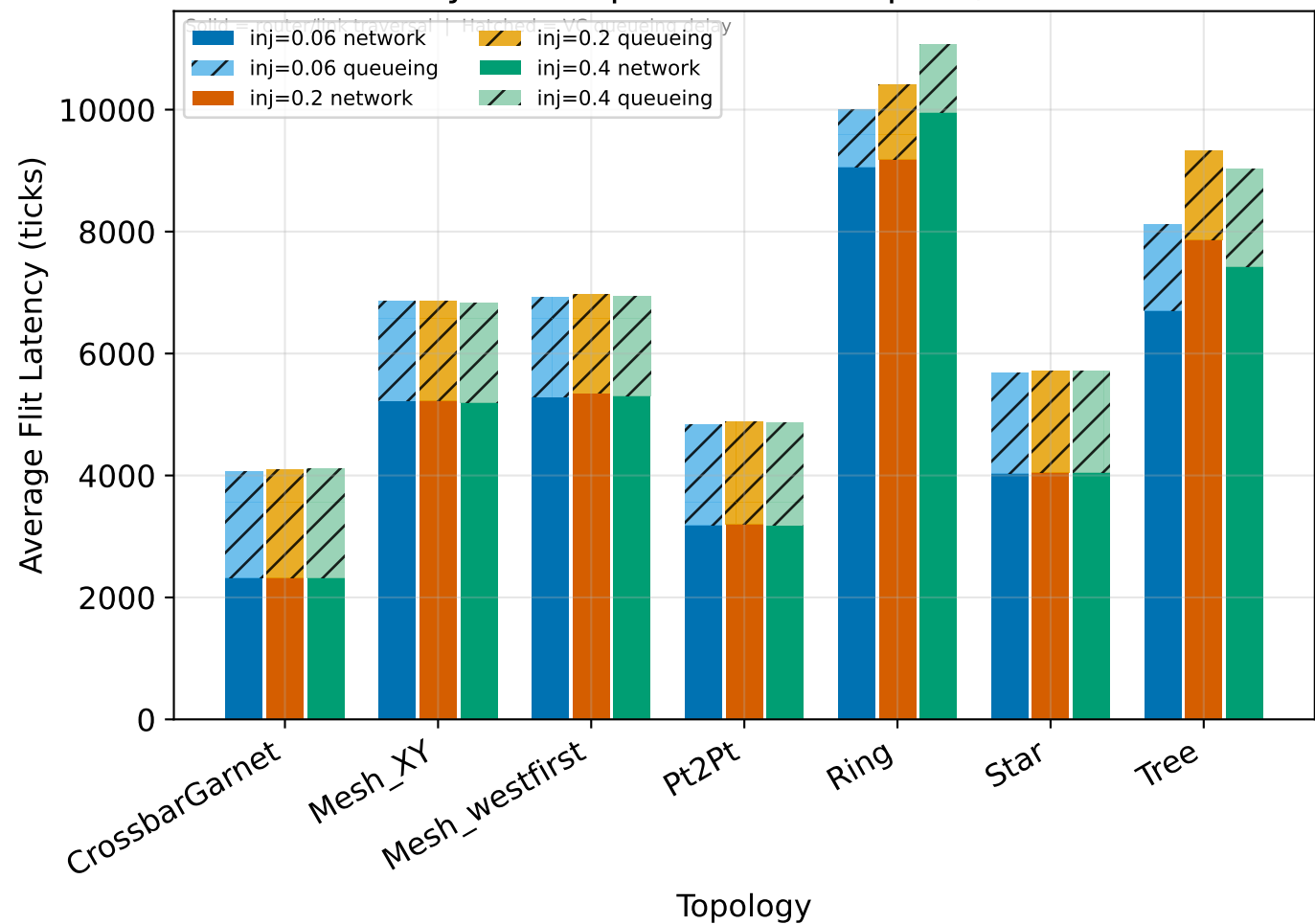
Latency Decomposition - transpose, 32 nodes
