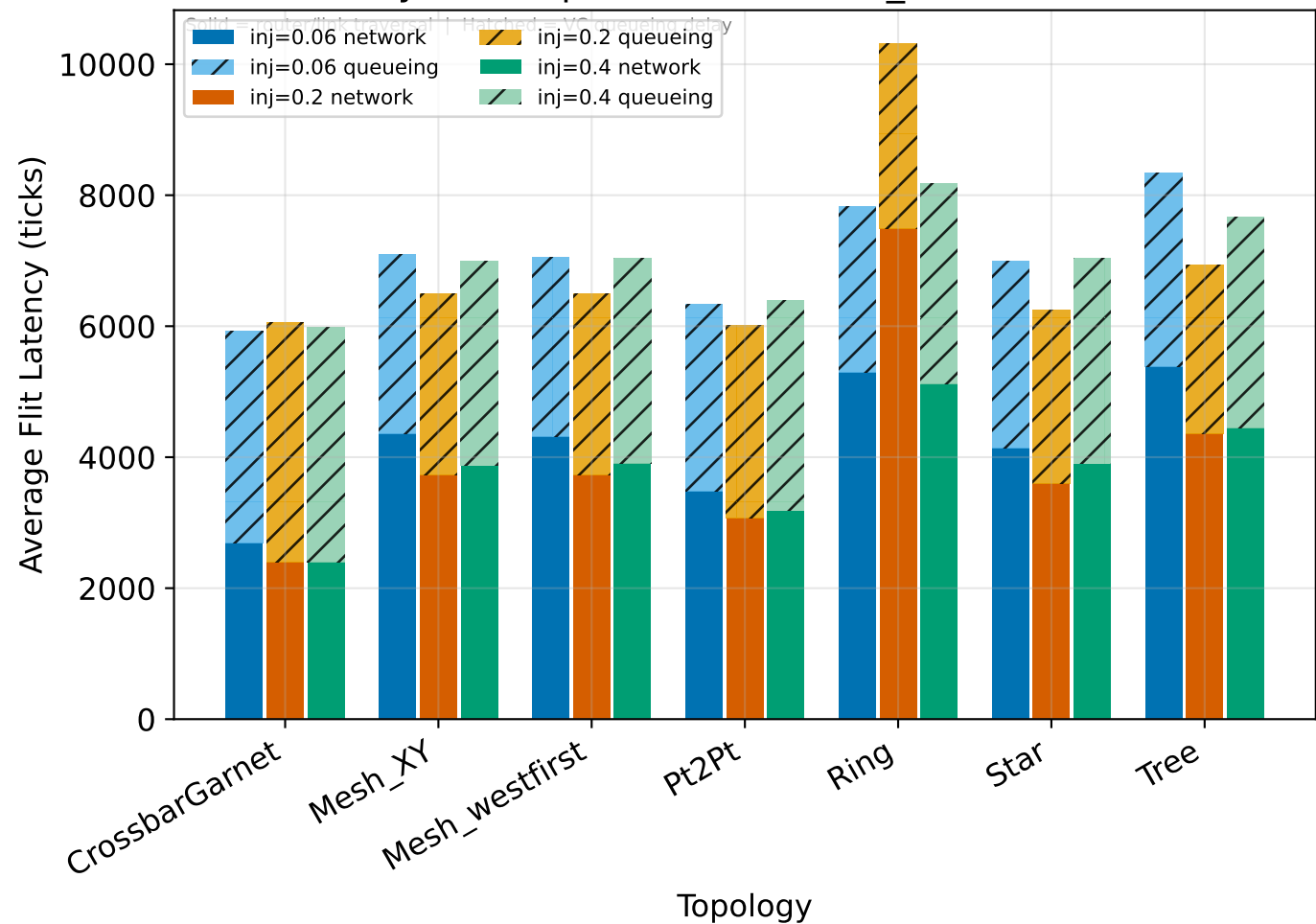
Latency Decomposition - uniform_random, 8 nodes
