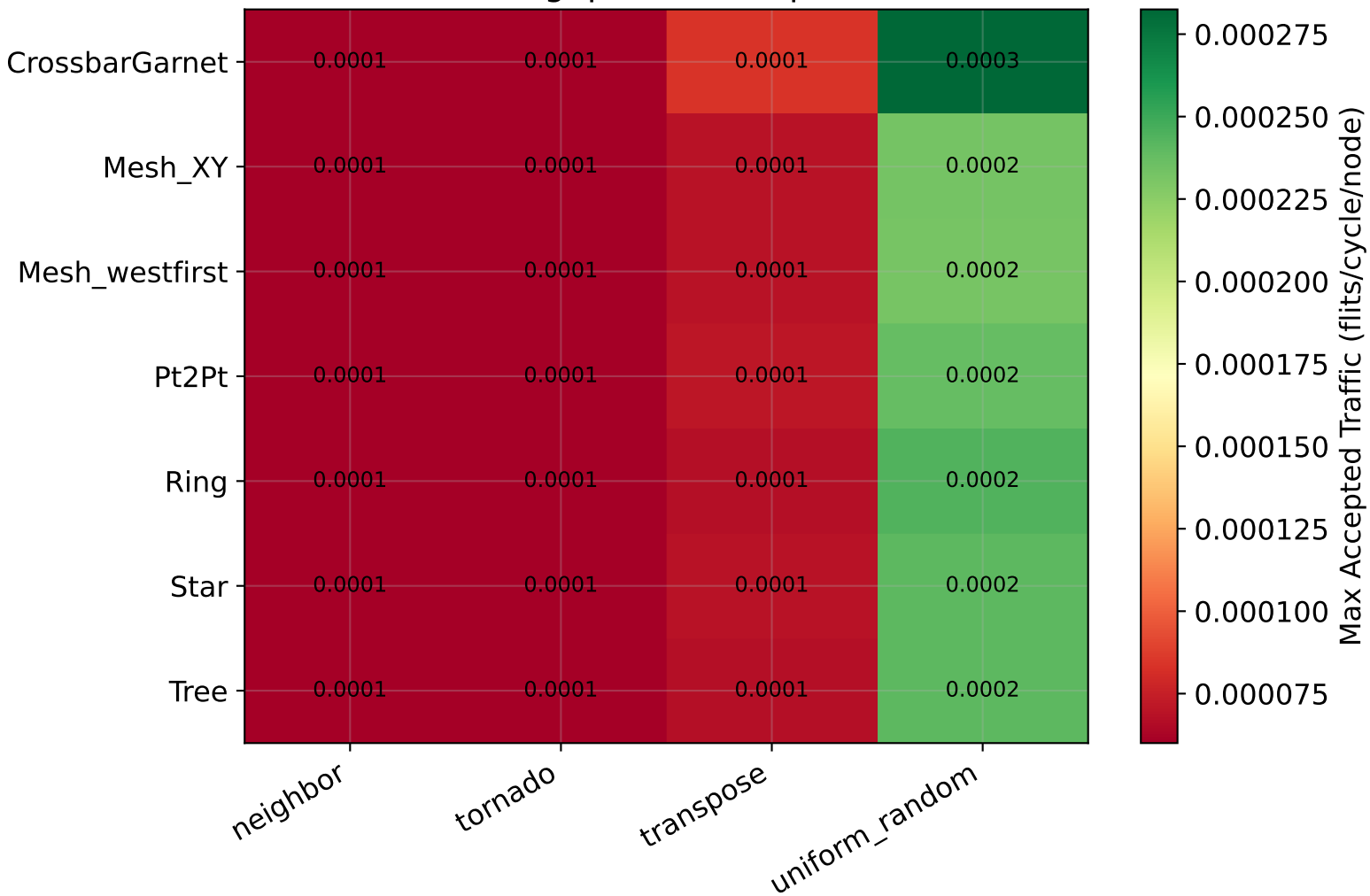
Peak Throughput Heatmap - 8 nodes
