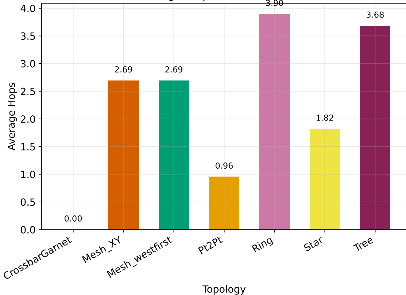
Average Hop Count - 32 nodes
