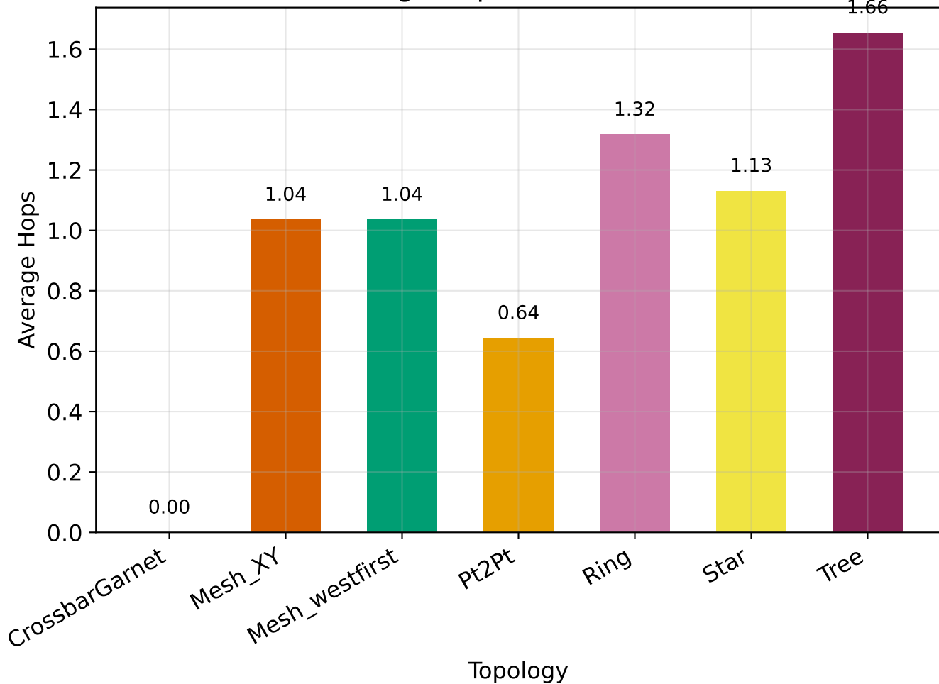
Average Hop Count - 8 nodes
