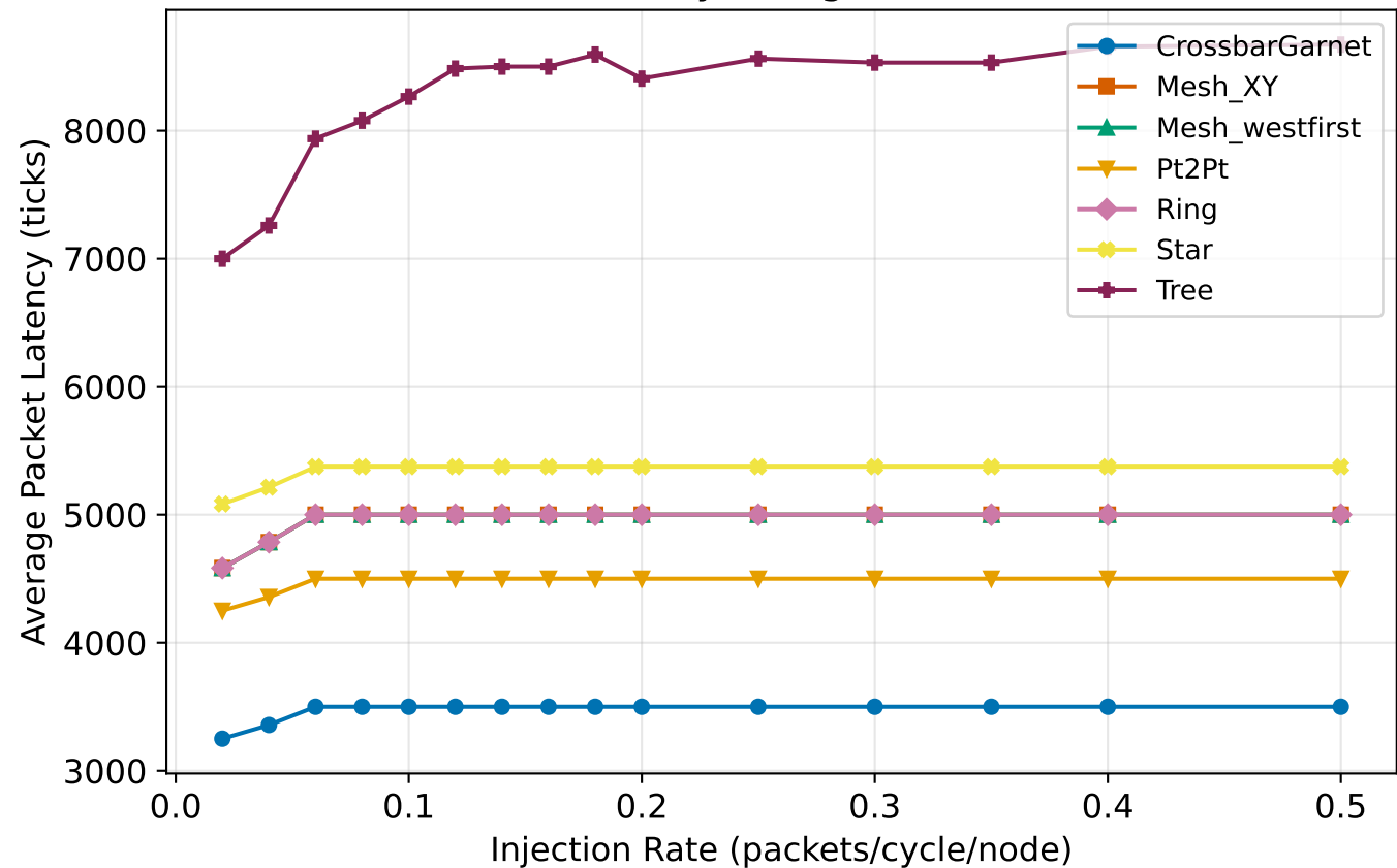
Packet Latency - neighbor, 16 nodes
