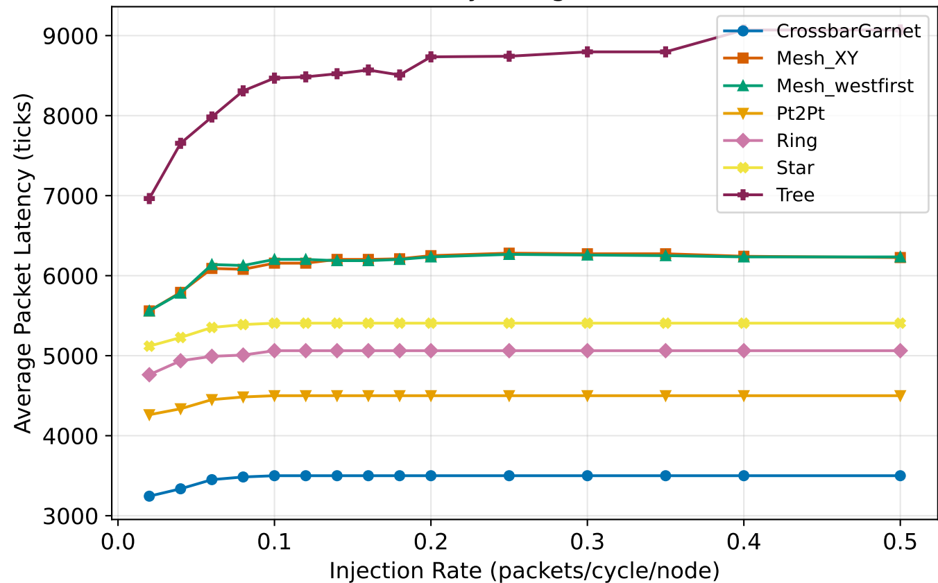
Packet Latency - neighbor, 32 nodes
