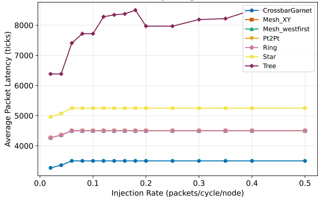
Packet Latency - neighbor, 8 nodes
