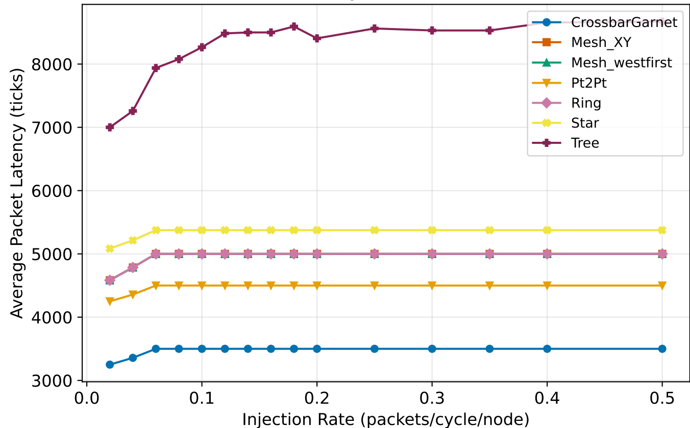
Packet Latency - tornado, 16 nodes
