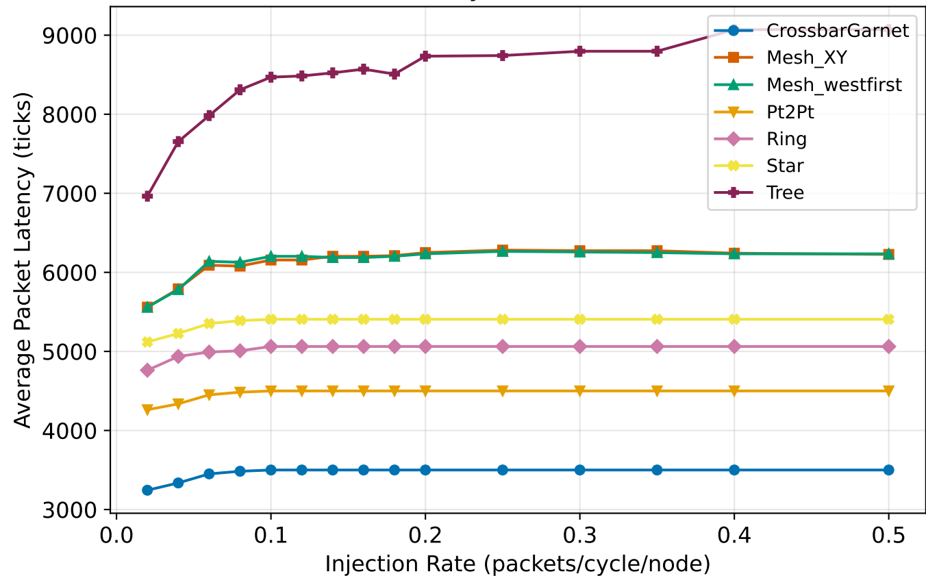
Packet Latency - tornado, 32 nodes
