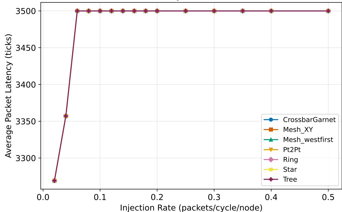
Packet Latency - tornado, 8 nodes
