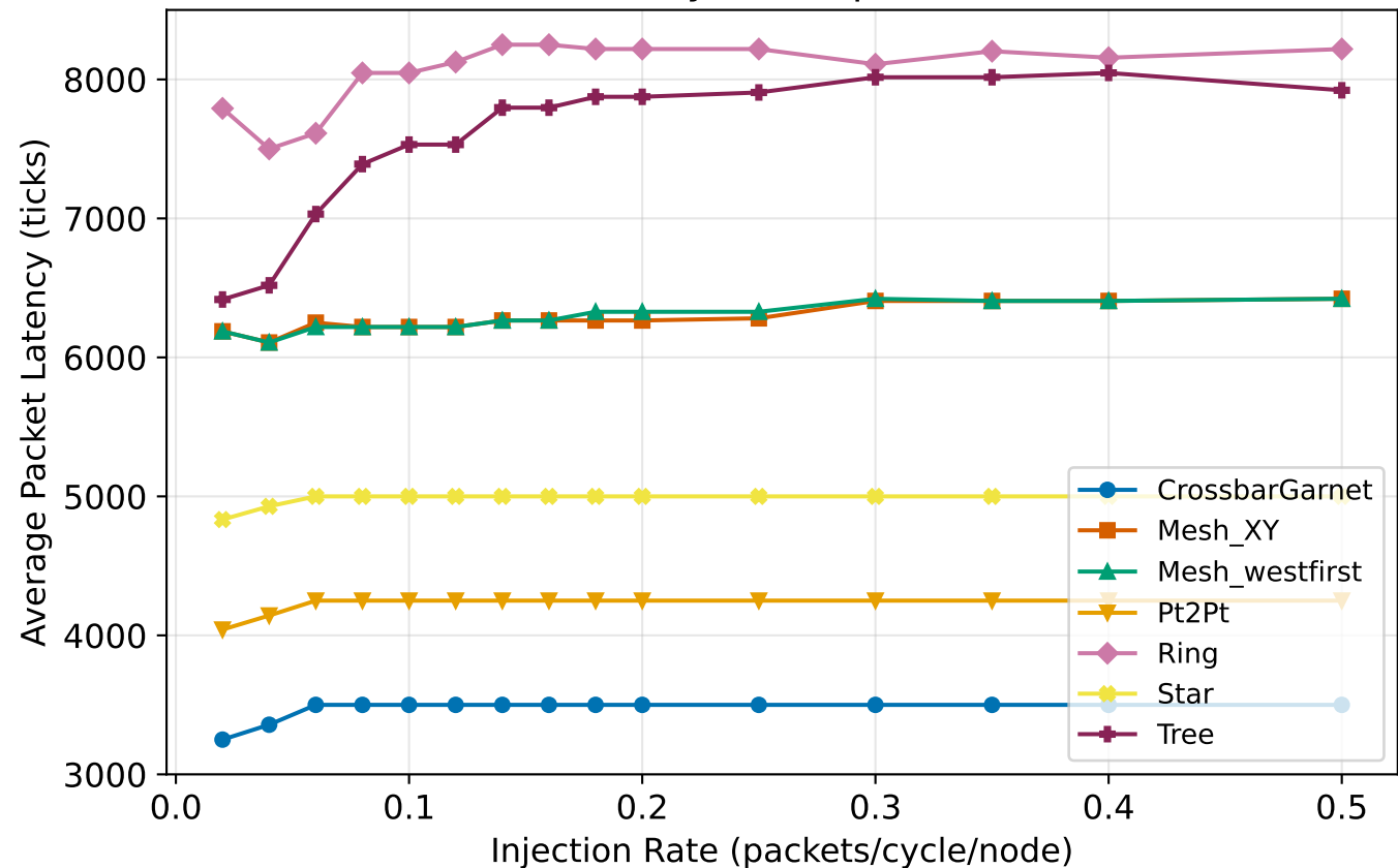
Packet Latency - transpose, 16 nodes
