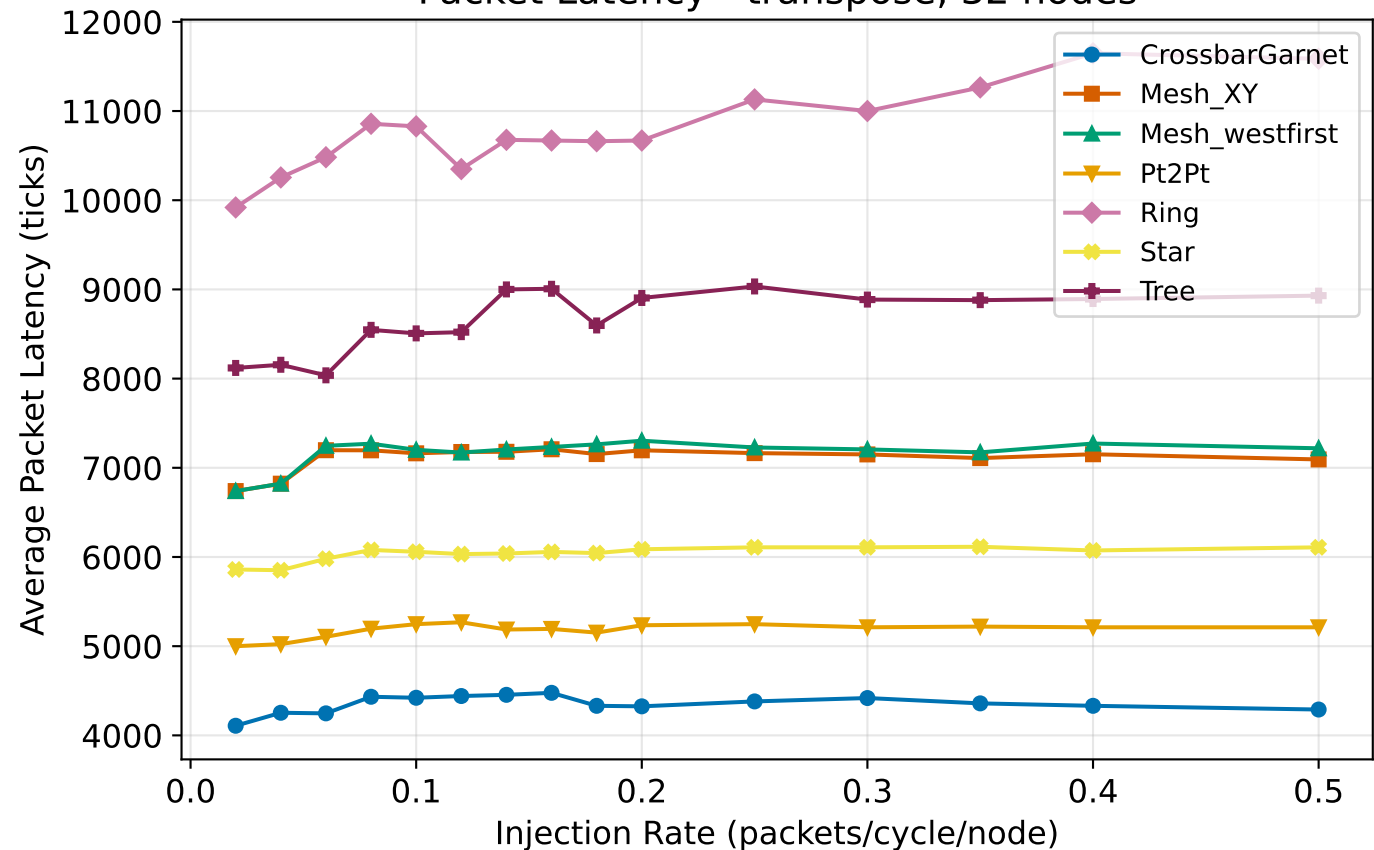
Packet Latency - transpose, 32 nodes
