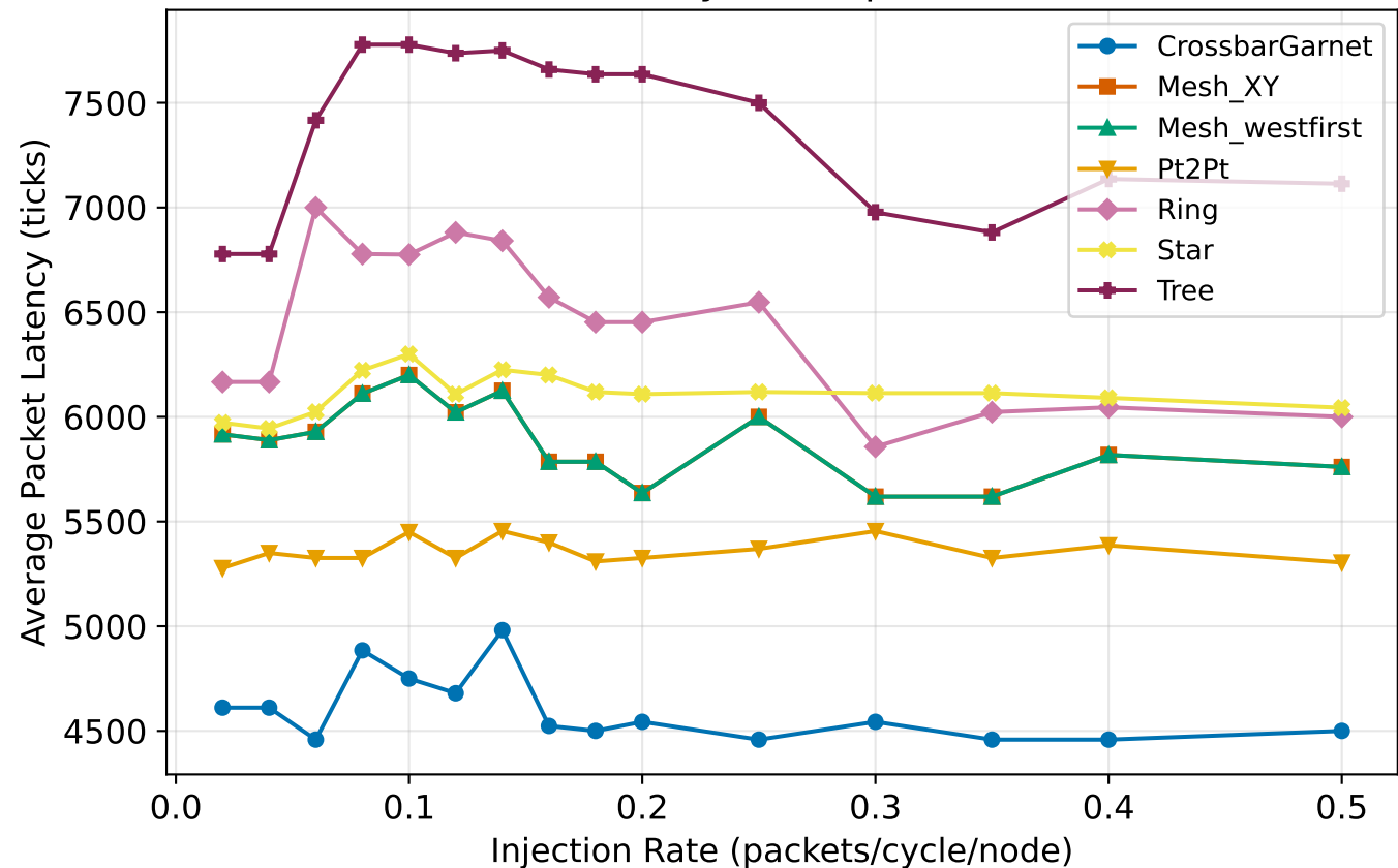
Packet Latency - transpose, 8 nodes
