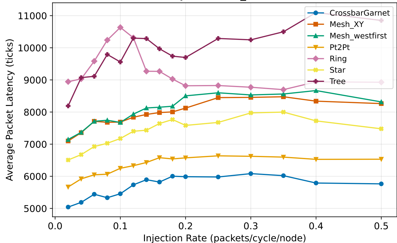
Packet Latency - uniform_random, 16 nodes
