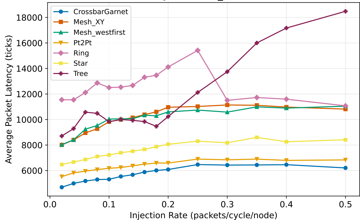
Packet Latency - uniform_random, 32 nodes
