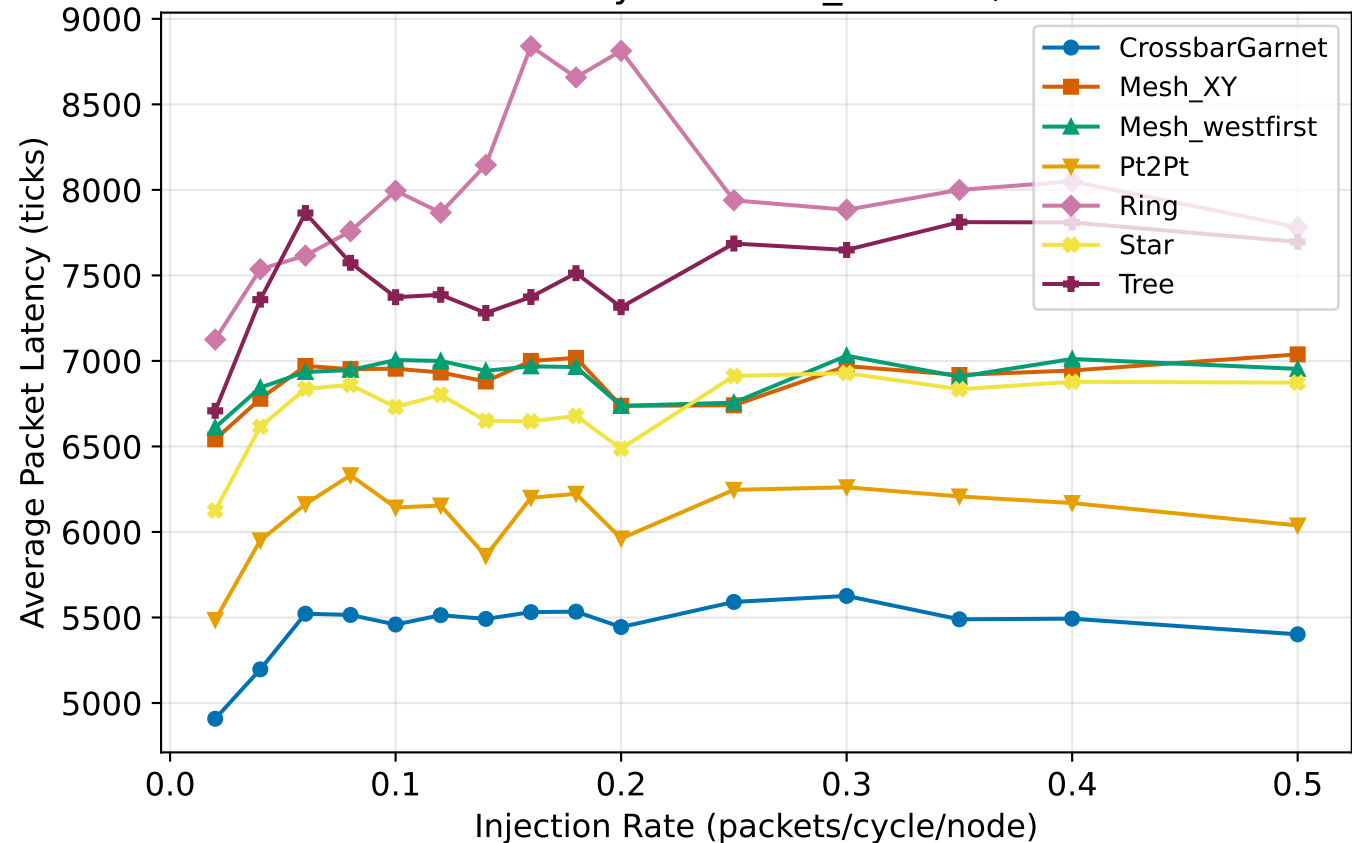
Packet Latency - uniform_random, 8 nodes
