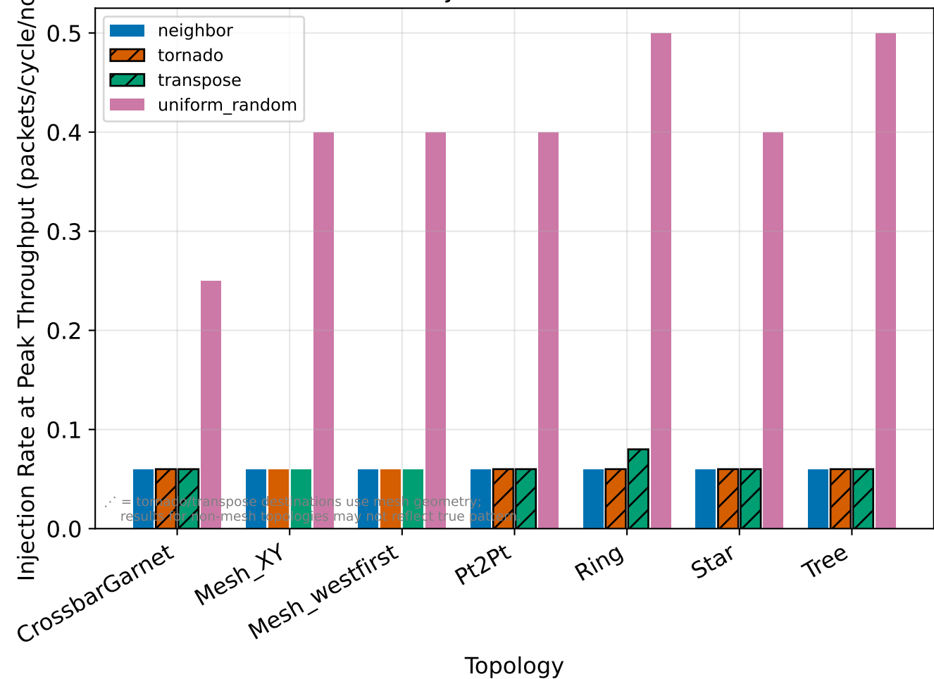
Saturation Injection Rate - 16 nodes
