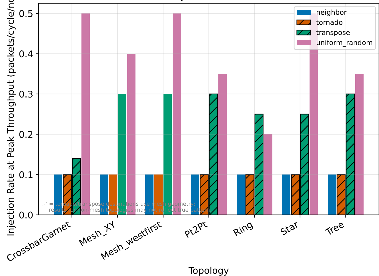
Saturation Injection Rate - 32 nodes
