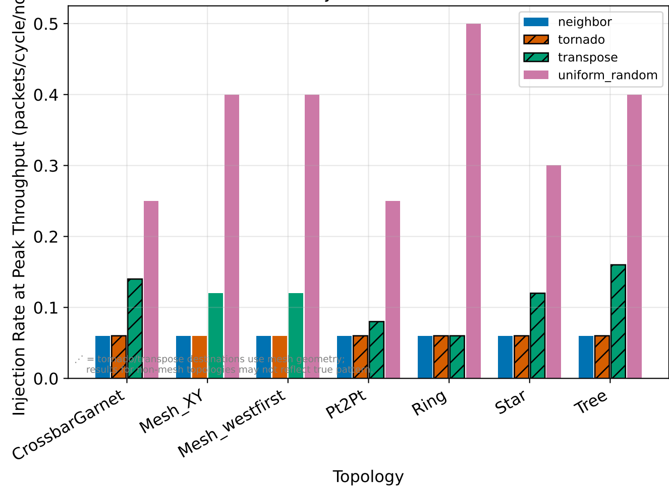
Saturation Injection Rate - 8 nodes
