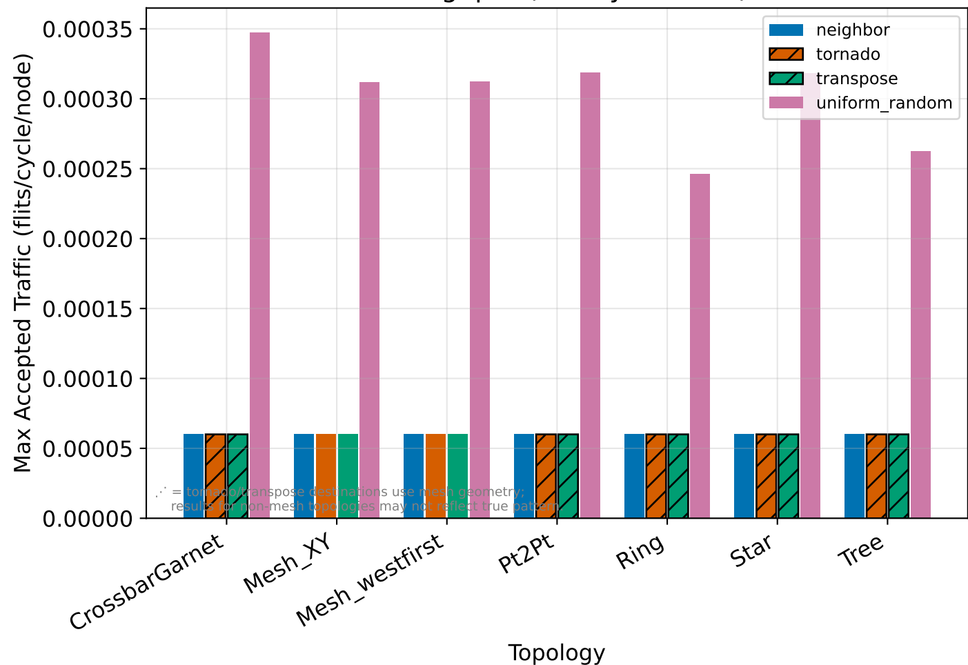
Saturation Throughput (flits/cycle/node) - 16 nodes
