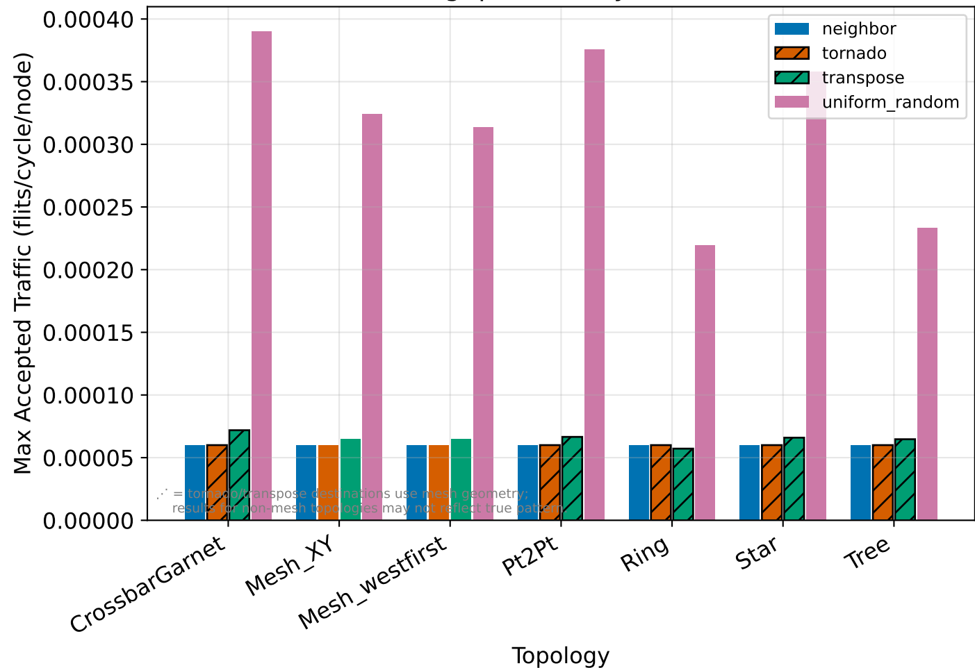
Saturation Throughput (flits/cycle/node) - 32 nodes
