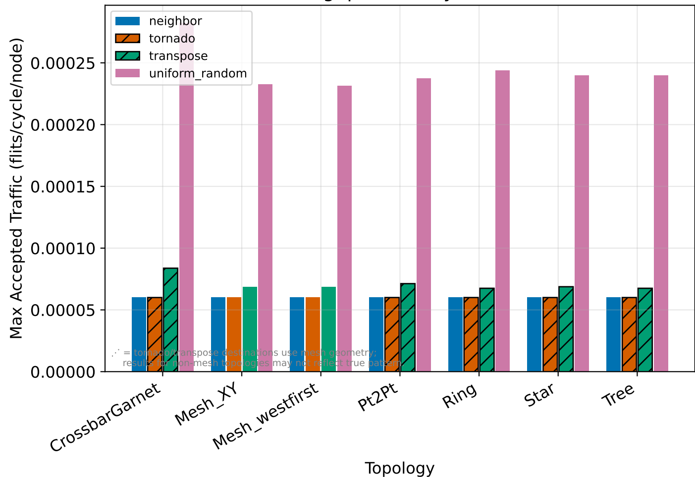
Saturation Throughput (flits/cycle/node) - 8 nodes
