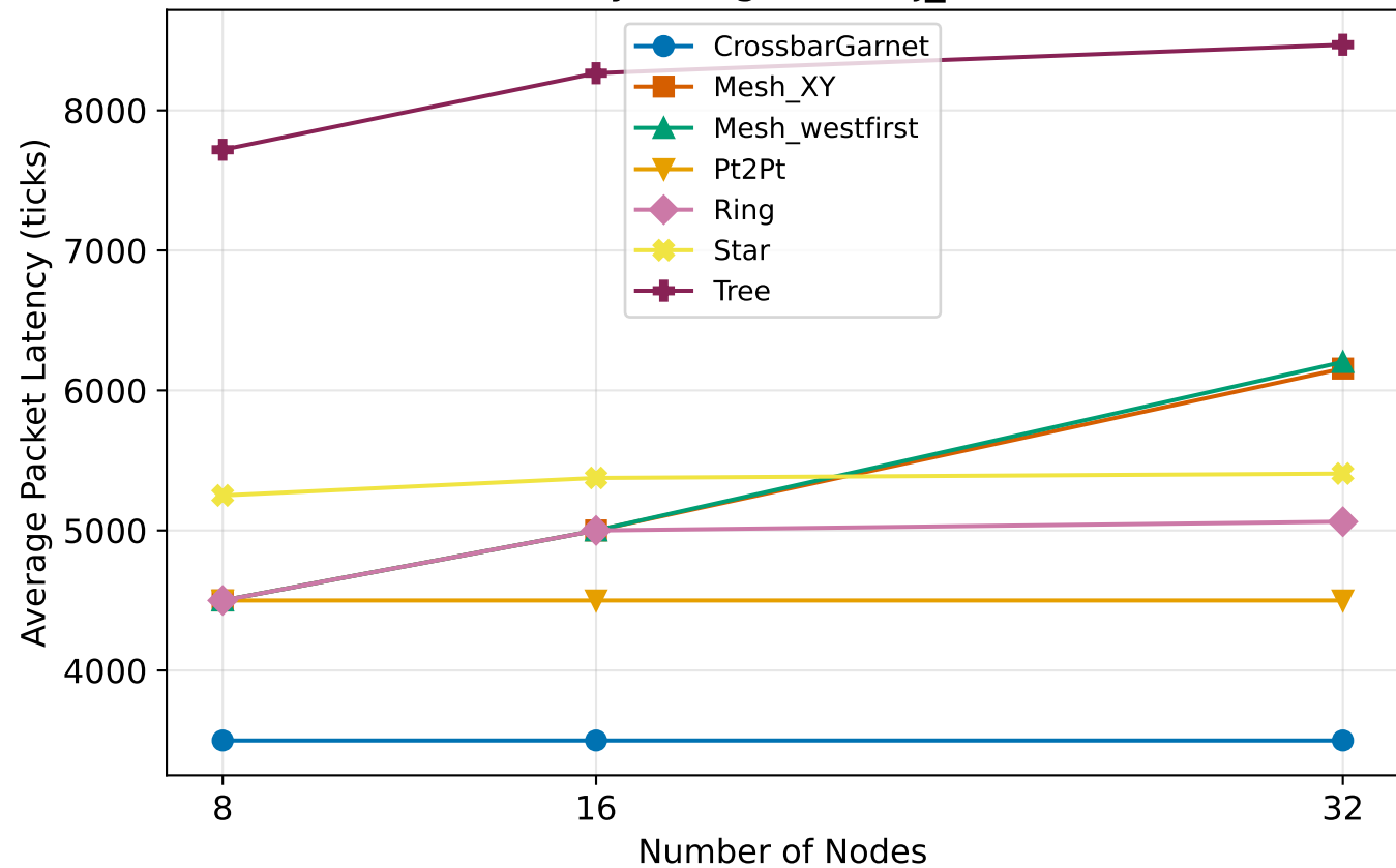
Scalability - neighbor (inj_rate=0.1)
