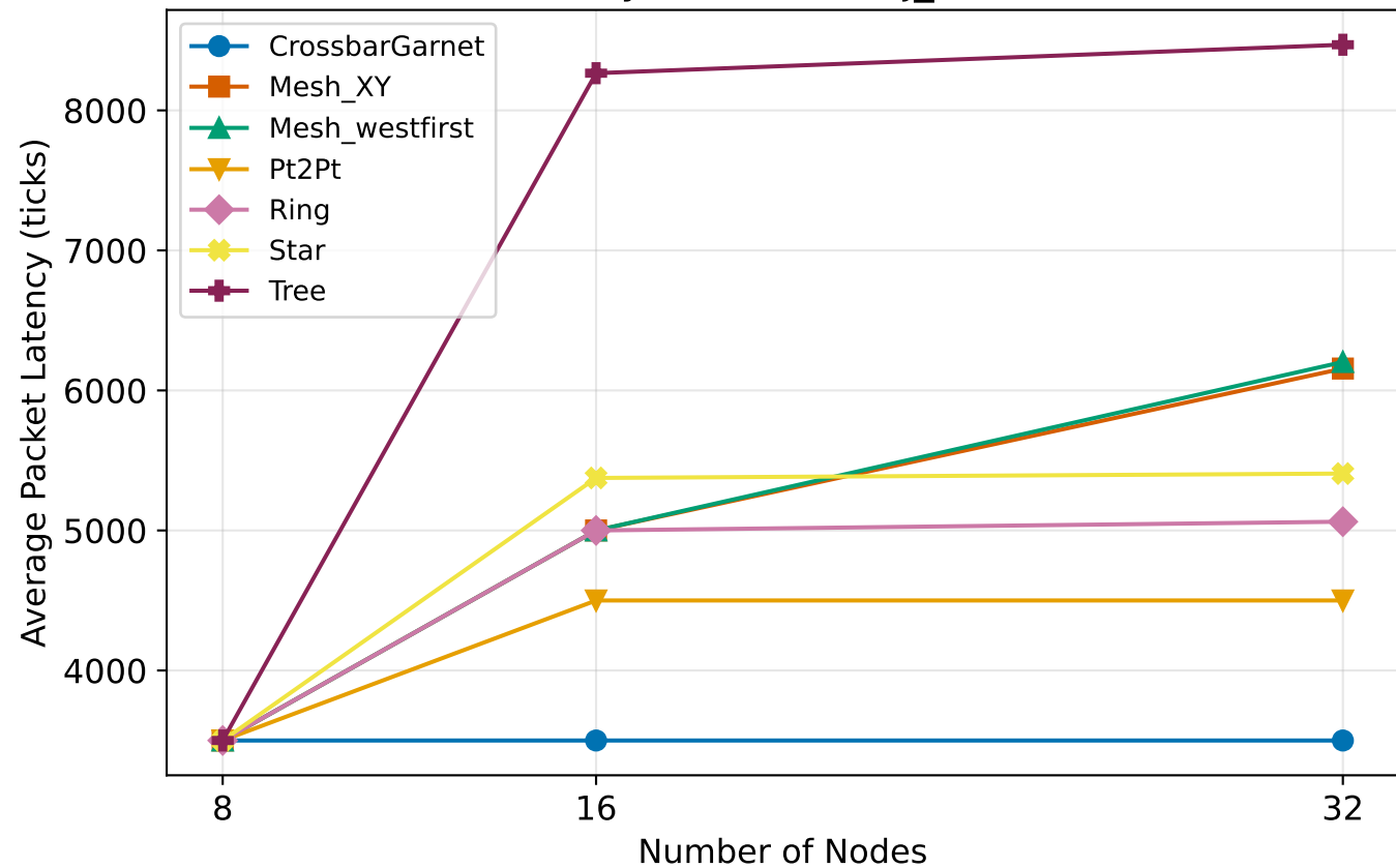
Scalability - tornado (inj_rate=0.1)
