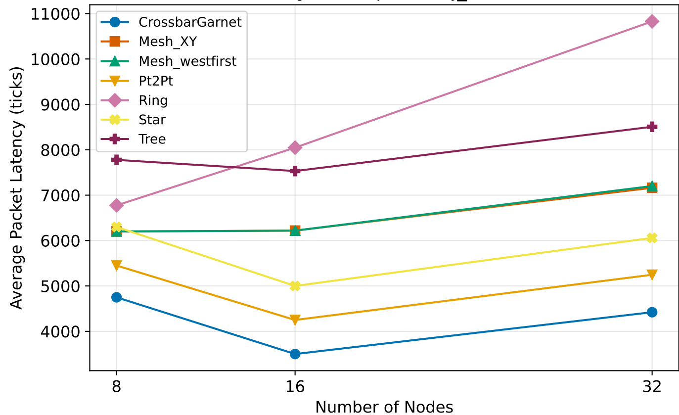
Scalability - transpose (inj_rate=0.1)
