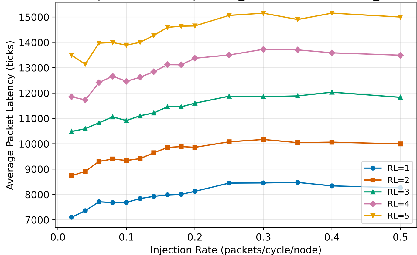
Sensitivity: Router Latency (Mesh_XY, 16 nodes, uniform_random)
