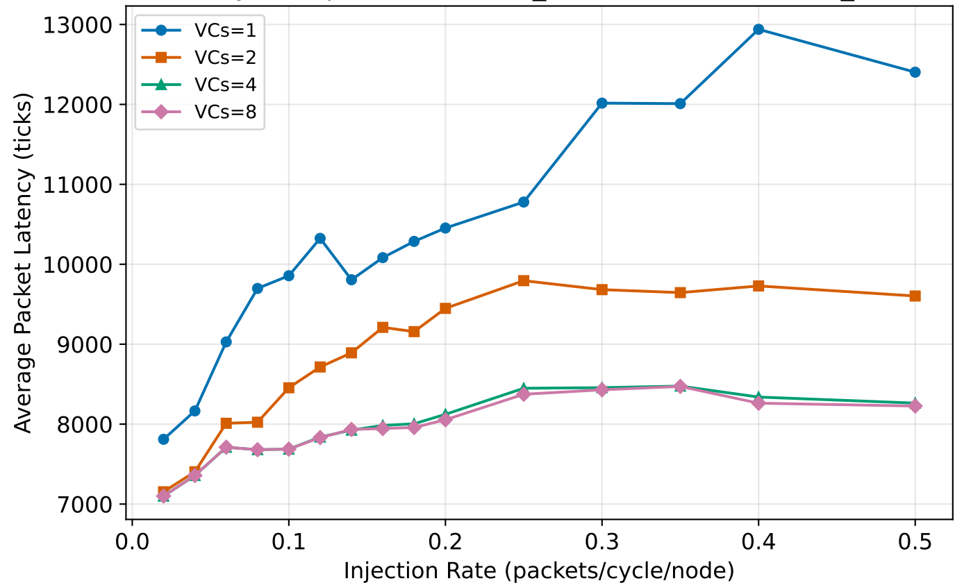
Sensitivity: VCs per VNet (Mesh_XY, 16 nodes, uniform_random)
