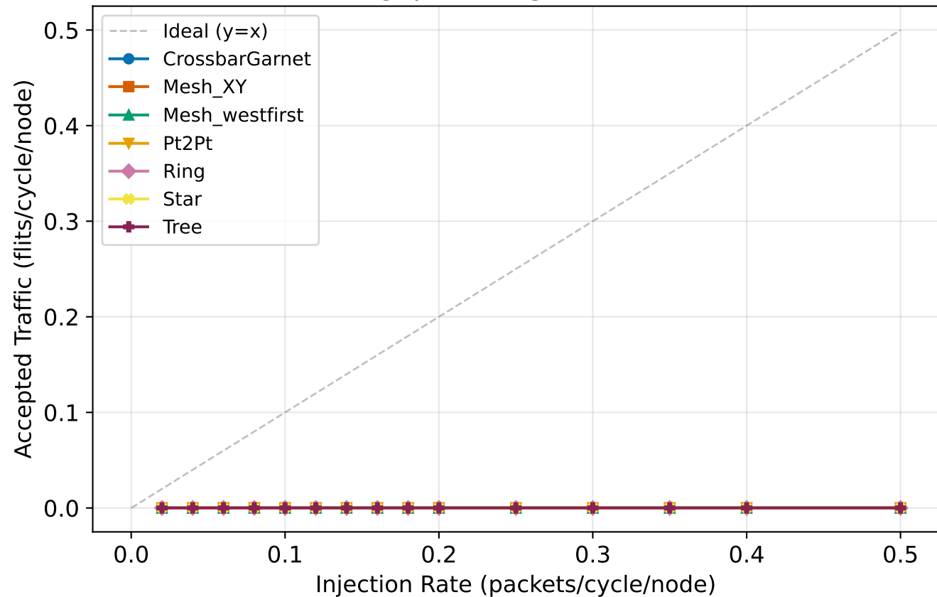
Throughput - neighbor, 8 nodes
