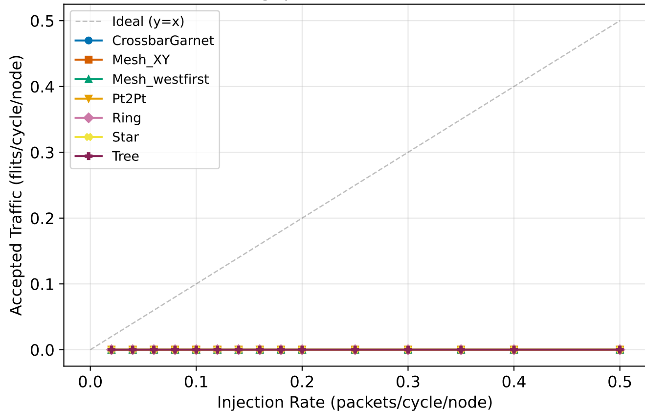
Throughput - tornado, 16 nodes
