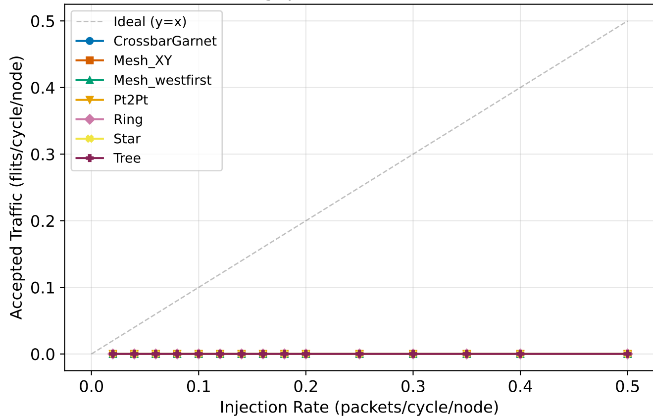
Throughput - tornado, 32 nodes
