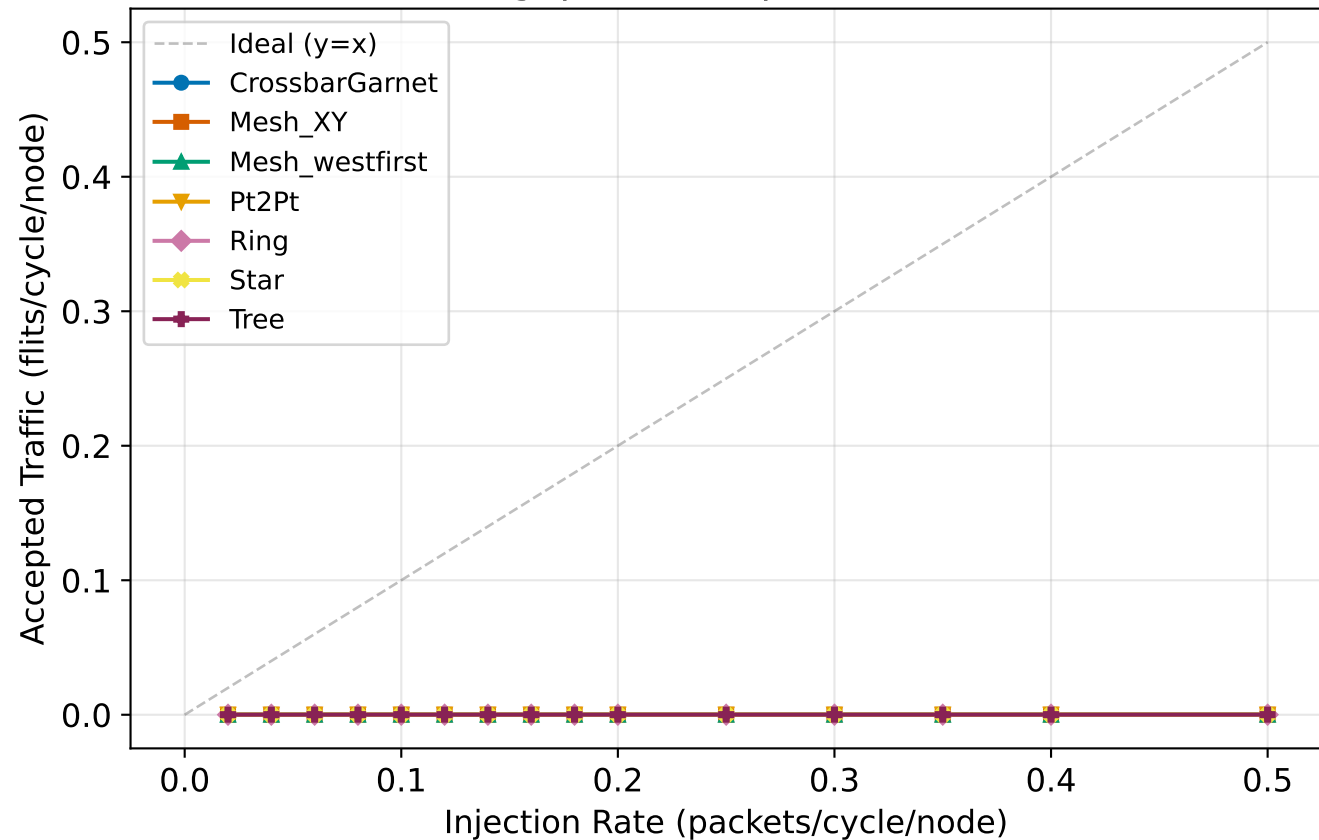
Throughput - transpose, 32 nodes
