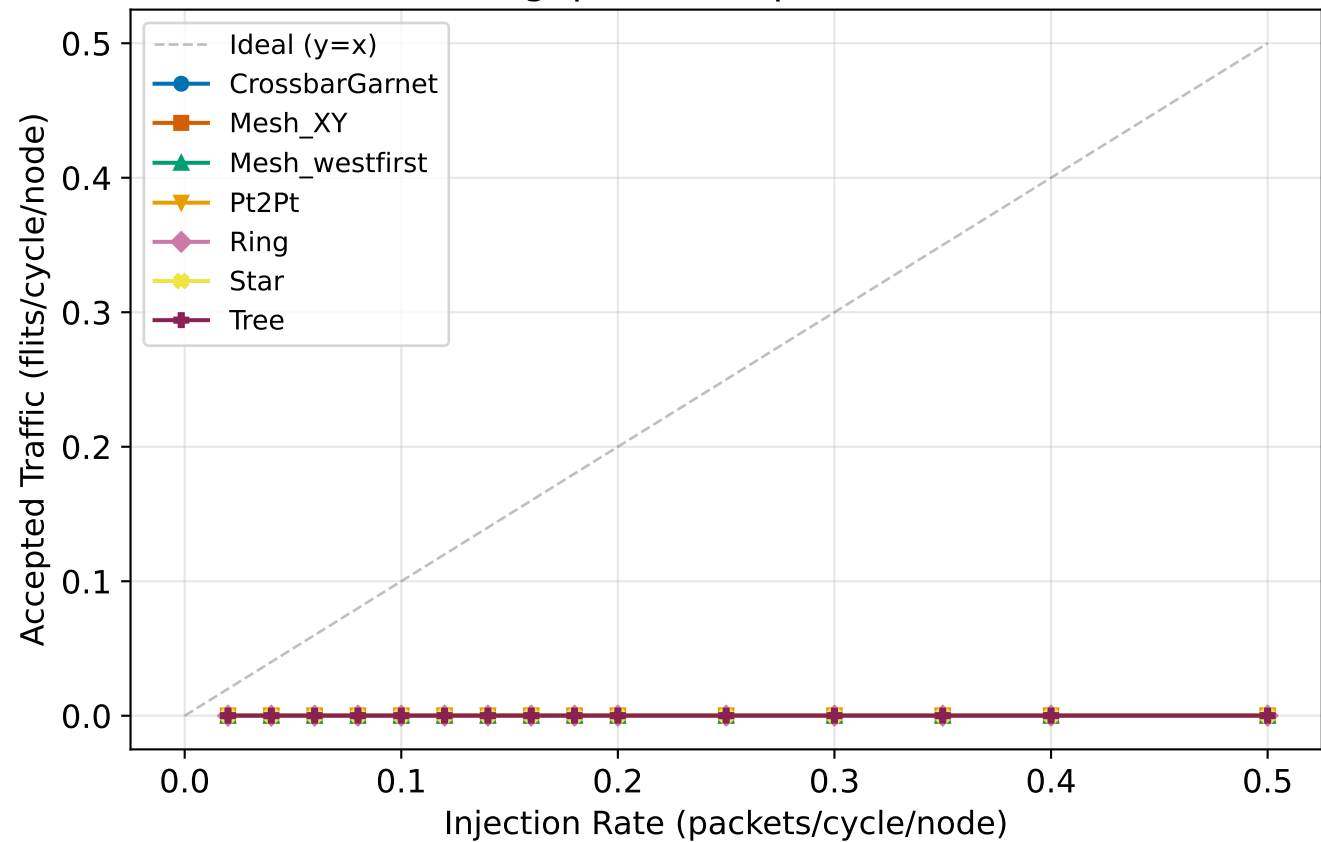
Throughput - transpose, 8 nodes
