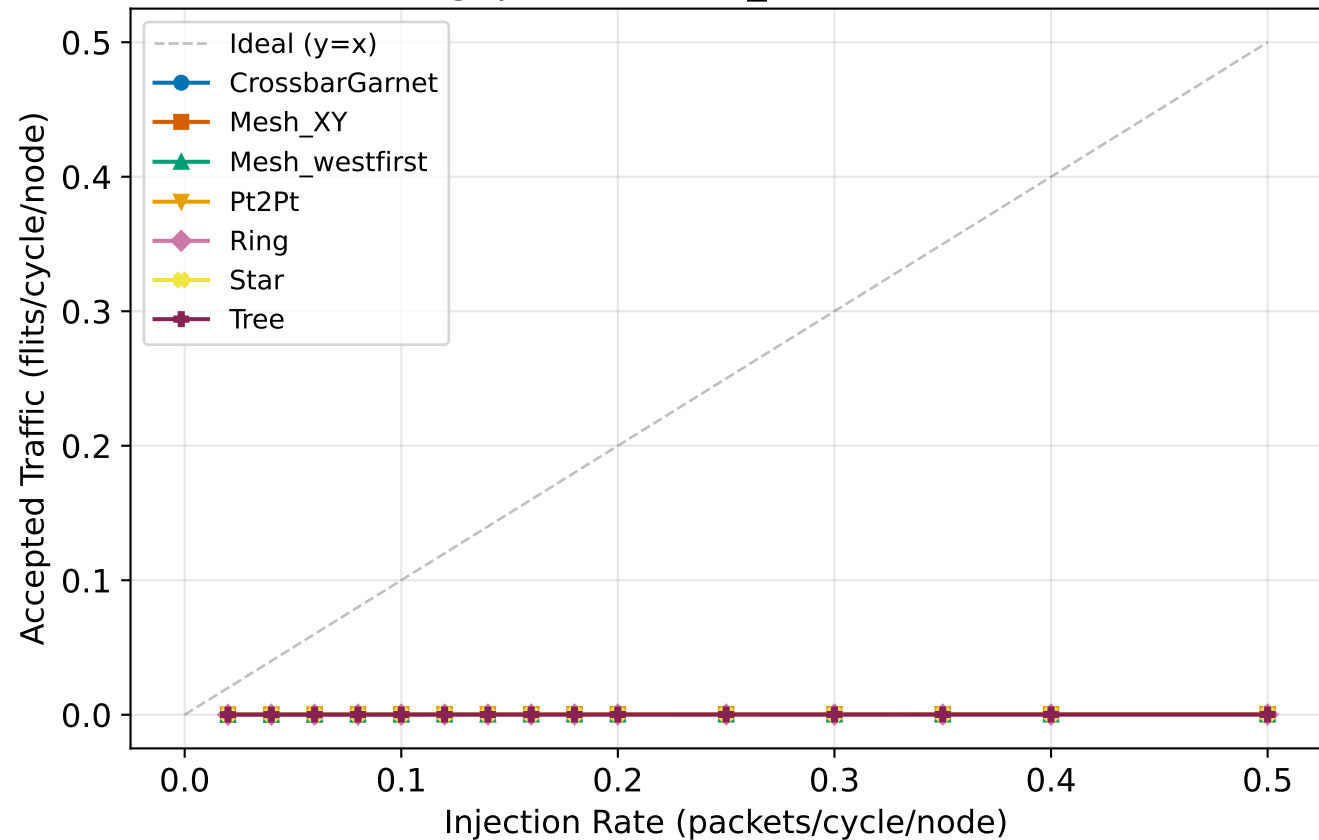
Throughput - uniform_random, 32 nodes
