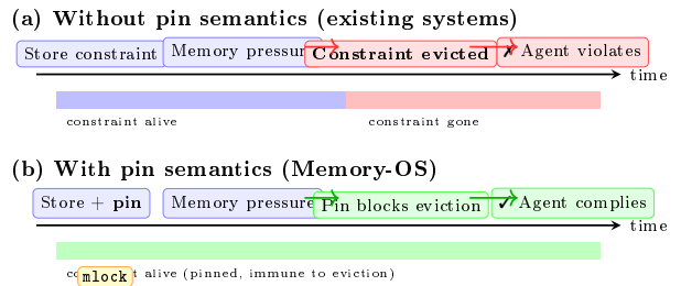
Figure 1: The pin-guarantee problem. (a) Existing systems evict constraints under memory pressure, causing agents to re-violate established rules. (b) Memory-OS’s mlock -inspired pin semantics guarantee constraint survival regardless of pressure.
