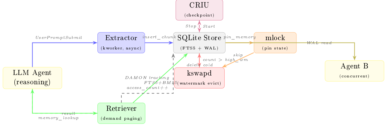
Figure 2: Memory-OS architecture as a data-flow diagram. Chunks flow through write (blue), retrieval (green), eviction (red), and checkpoint (purple) paths. Pin state (orange) blocks eviction; WAL mode enables concurrent multi-agent access (yellow). OS primitive analogs annotated.
