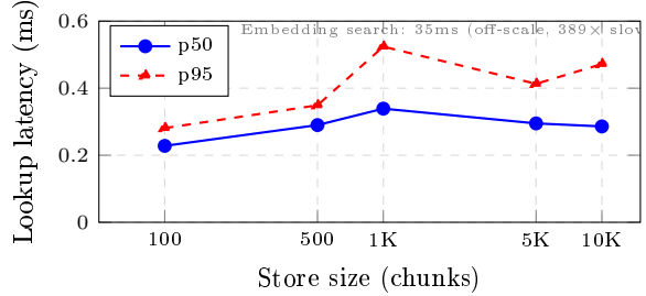
Figure 4: FTS5 lookup latency vs. store size. Sub-millisecond at all scales; embedding search (35ms, off-scale) shown for reference.
