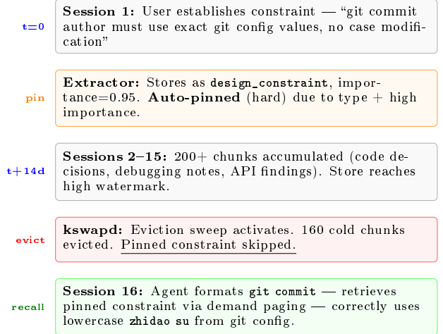
Figure 5: Case study from production deployment. A constraint pinned in Session 1 survives 14 days of memory pressure (160 evictions) and is correctly recalled via demand paging in Session 16, preventing a previously-observed agent error.
