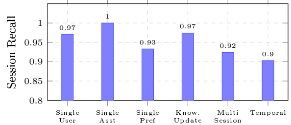
Figure 3: LongMemEval session recall by question type. Temporal reasoning (requiring time-reference matching) is the weakest category for lexical retrieval.
