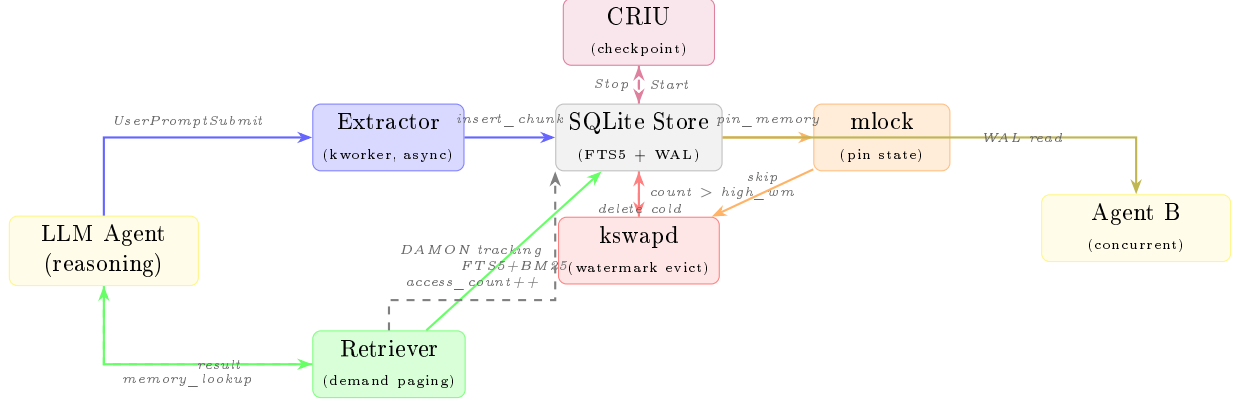
Figure 2: 0CompactMem architecture as a data-flow diagram. Chunks flow through write (blue), retrieval (green), eviction (red), and checkpoint (purple) paths. Pin state (orange) blocks eviction; WAL mode enables concurrent multi-agent access (yellow). OS primitive analogs annotated.
