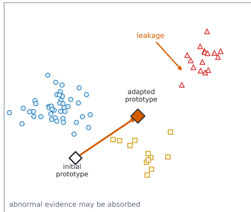
Direct TTA: prototype drift
