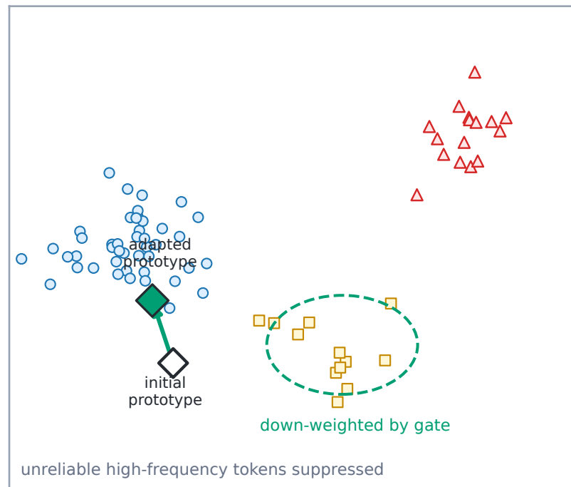
Ours: wavelet-gated update
