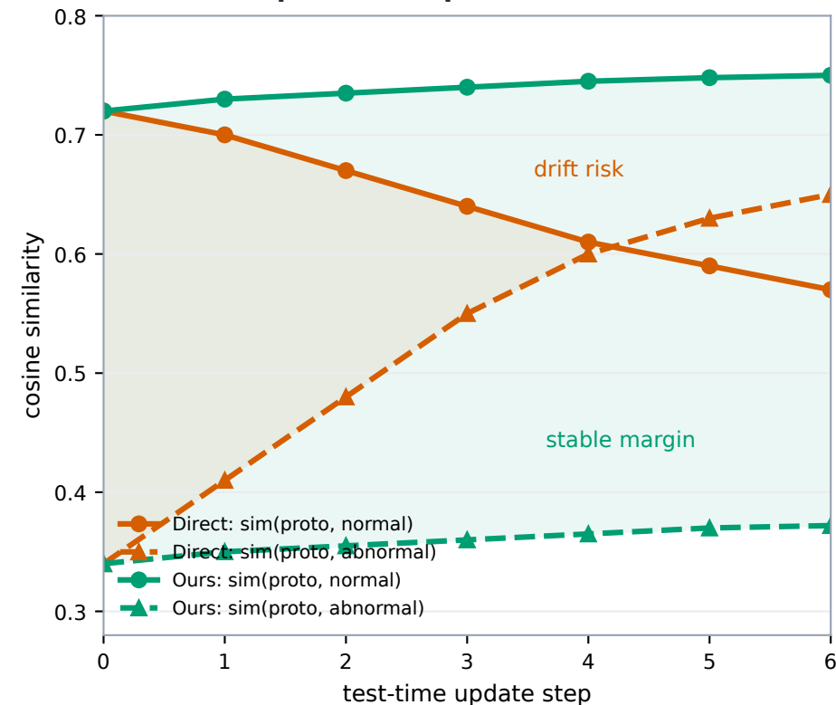
Expected adaptation behavior
