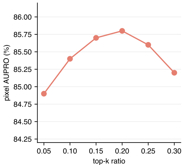
(a) top-k
