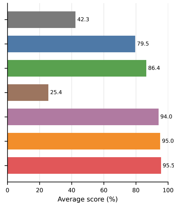
Pixel-AUROC
