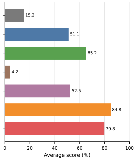
Pixel-AUPRO
