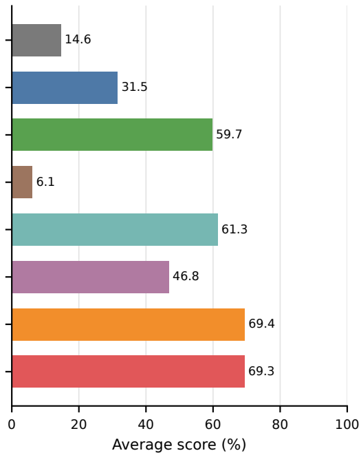
Pixel-AUPRO
