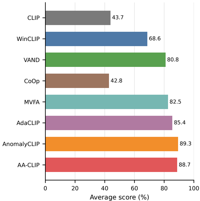
Pixel-AUROC
