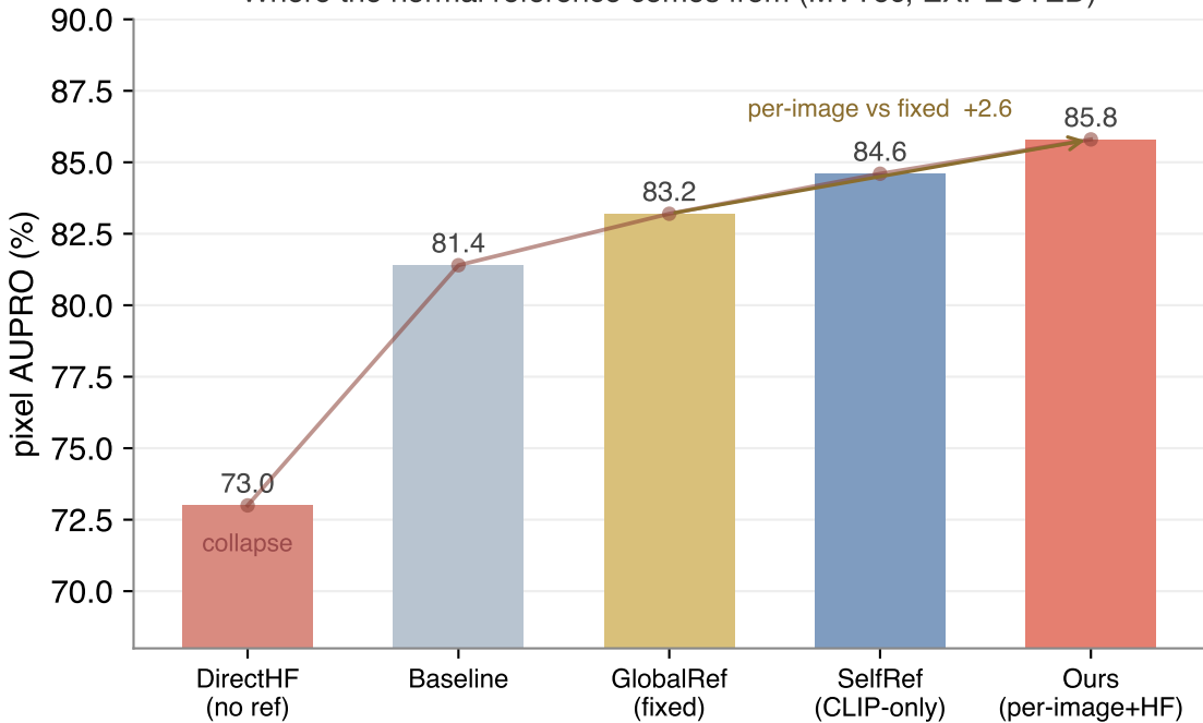
Where the normal reference comes from (MVTec, EXPECTED)
