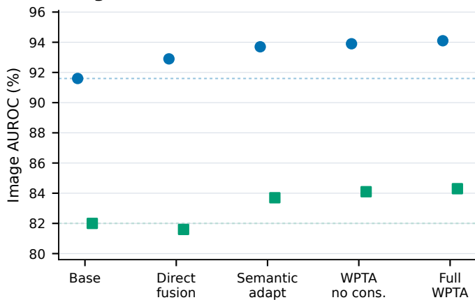
c Image AUROC
