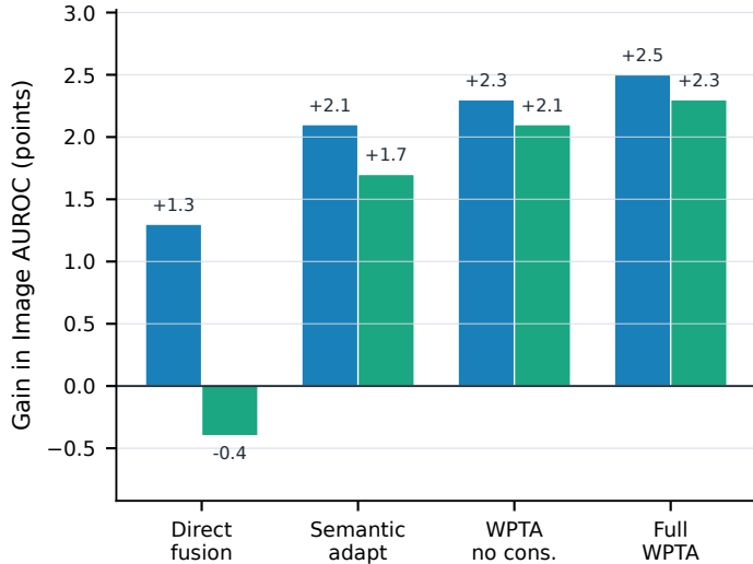
b Image AUROC: component gain
