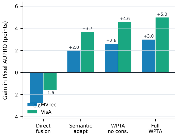
a Pixel AUPRO: component gain
