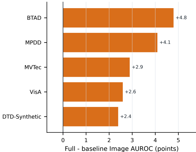
b Image AUROC: dataset gain
