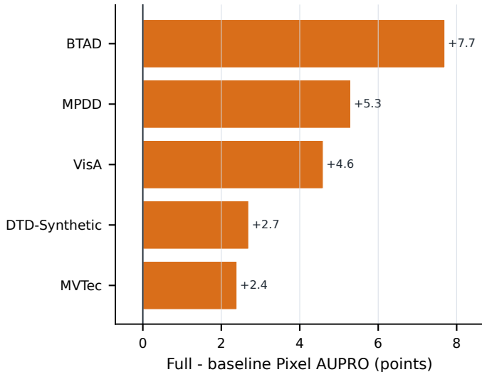
a Pixel AUPRO: dataset gain
