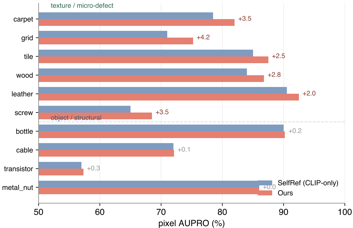
Gain concentrates on texture classes (MVTeC, EXPECTED)
