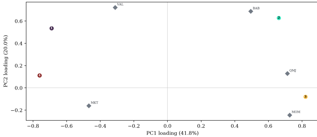
Figure: catalogue factors are numbered by directed-Sharpe index; attribution controls are named; N=212 common months.
