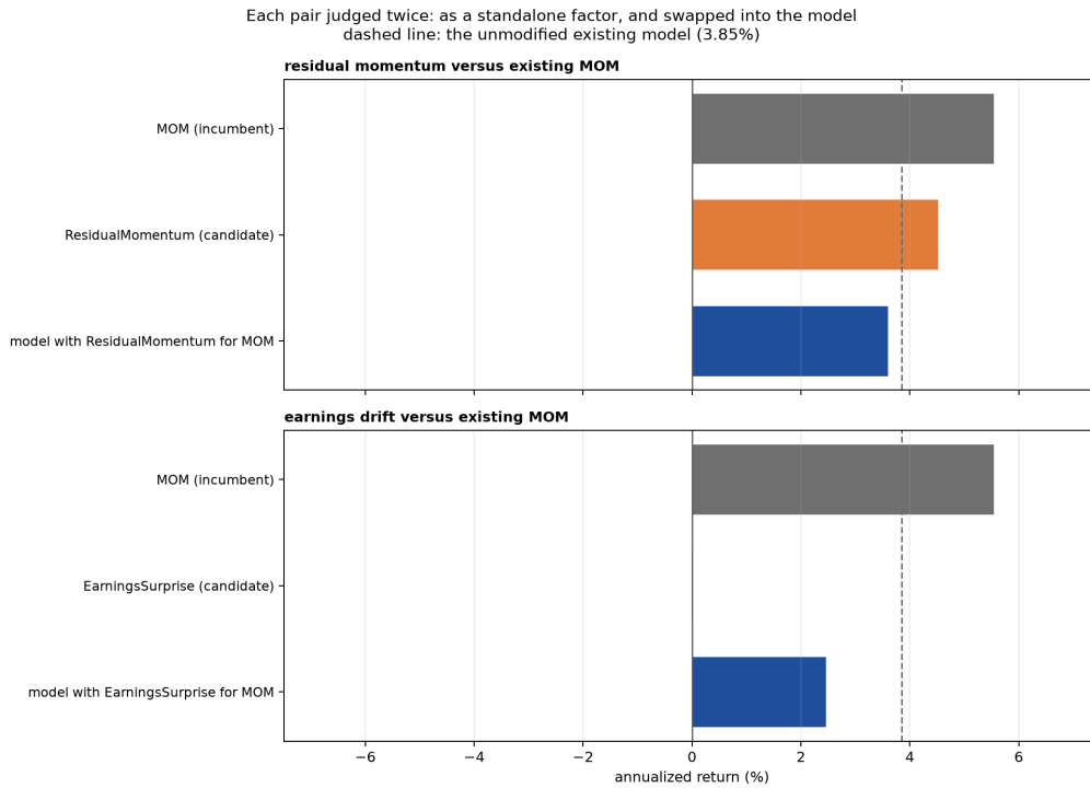
Figure 7: Each pair judged twice: the incumbent factor against the candidate standing alone, then the model with the candidate swapped in. The dashed line is the unmodified existing model.
