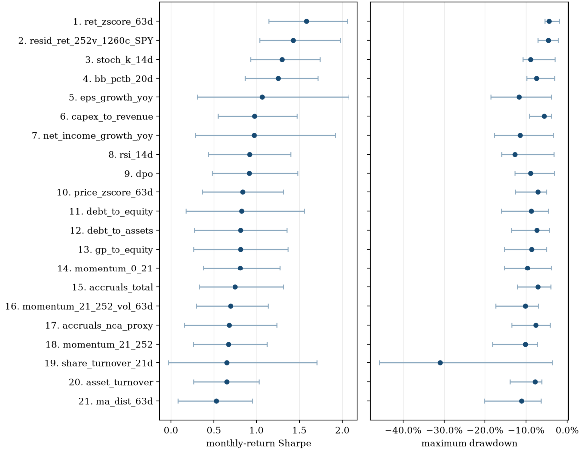
Figure: point estimates and paired stationary-bootstrap 95% intervals.
