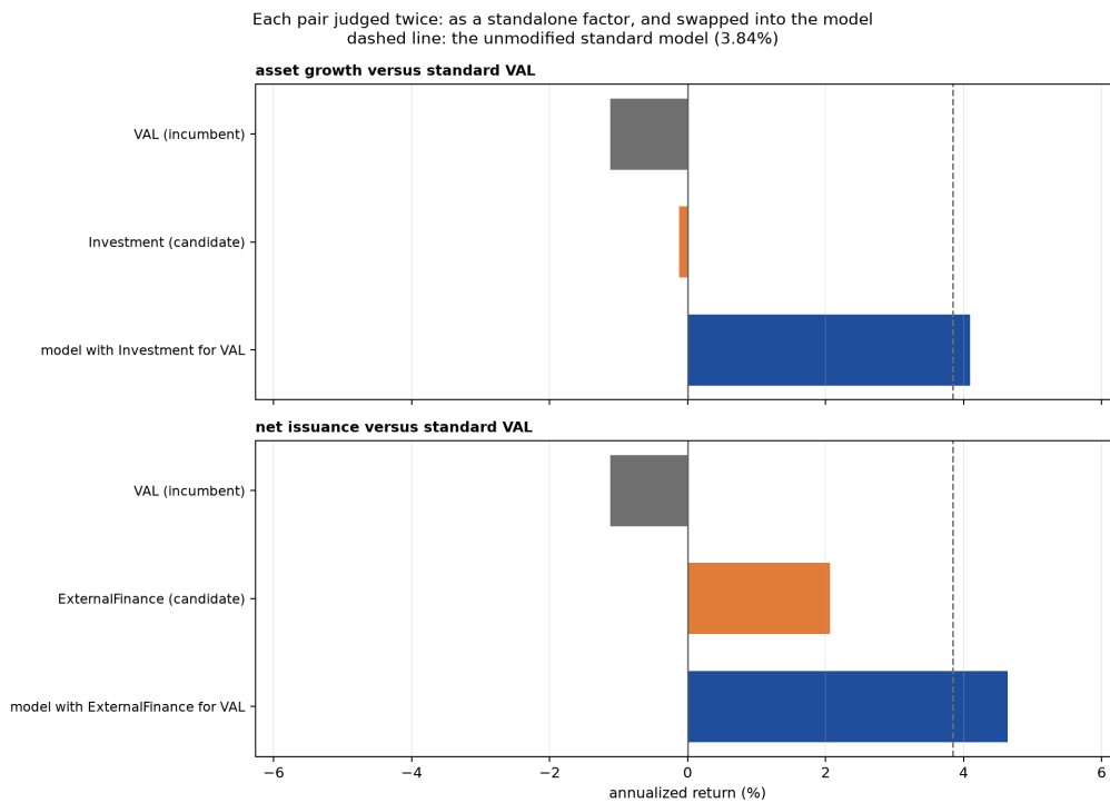
Figure 7: Each pair judged twice: the incumbent factor against the candidate standing alone, then the model with the candidate swapped in. The dashed line is the unmodified standard model.
